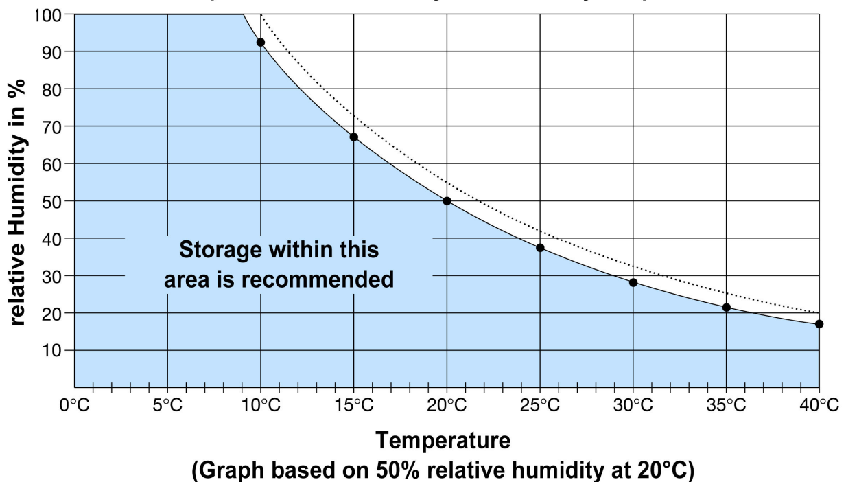
Graph shows safe storage conditions at different temperatures and depicts how rel humidity is affected by temperature
